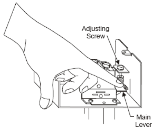
Figure 8 Minimum Adjustment
