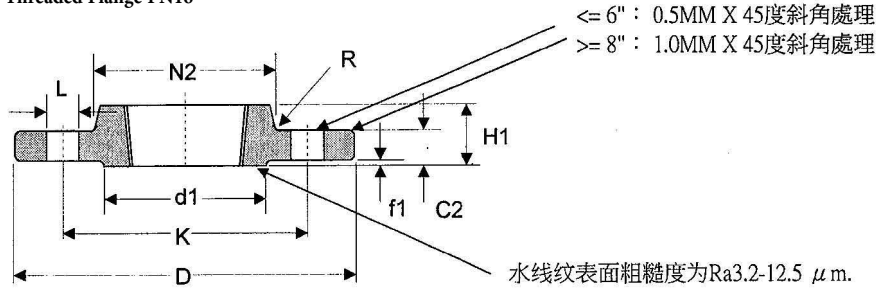
"HL" Threaded Flange PN16
