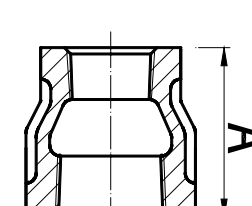
Reducing Socket
