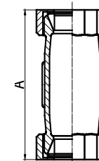
Long Compression Coupling
