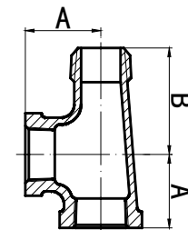
Service Tee
