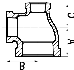
Reducing Tee
